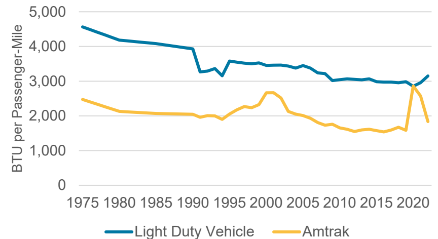
Figure 2.72 Passenger Mode Energy Intensity per Passenger Mile
