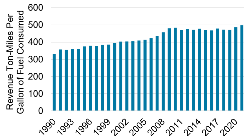
Figure 2.70 Class I Rail Freight Fuel Efficiency
