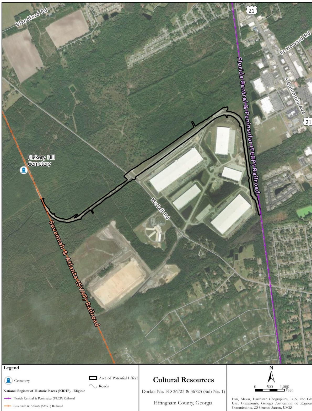
Figure 3-9 Cultural Resources
