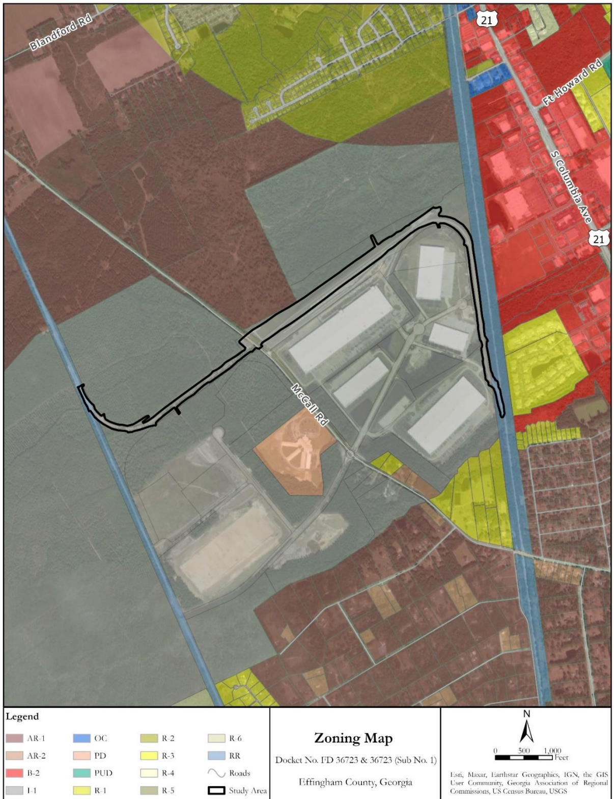
Figure 3-1 Zoning Map
