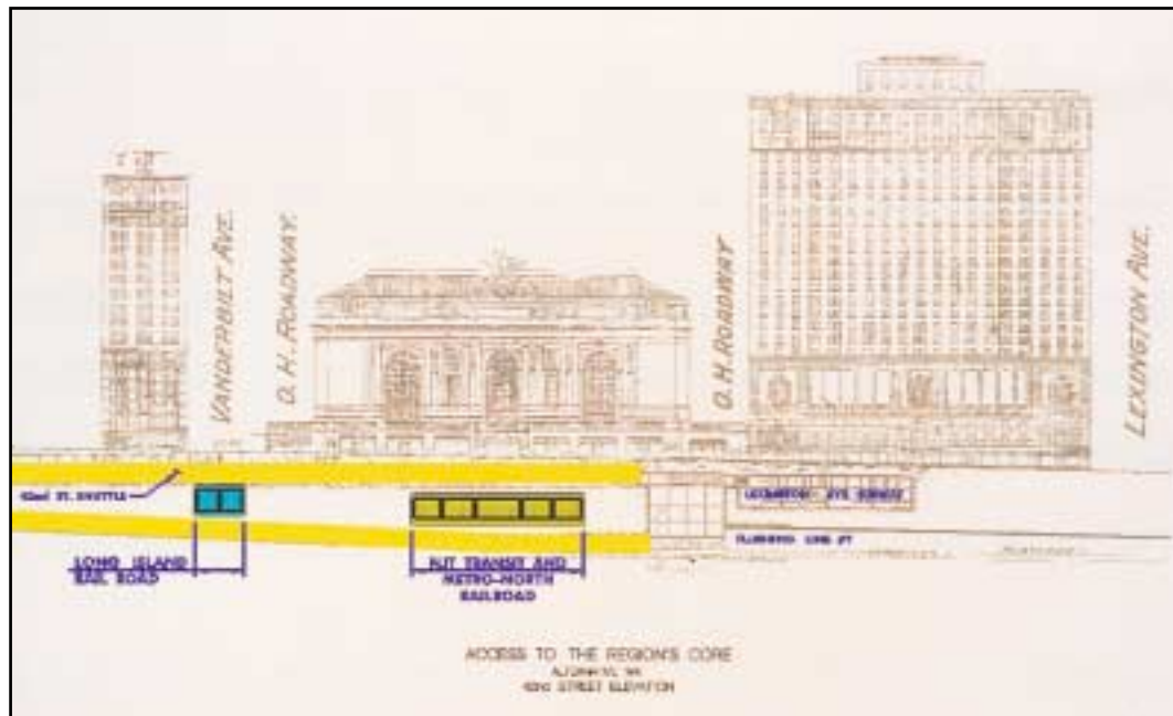
Figure 10 Alternative AA Grand Central Break Out at 42nd Street
