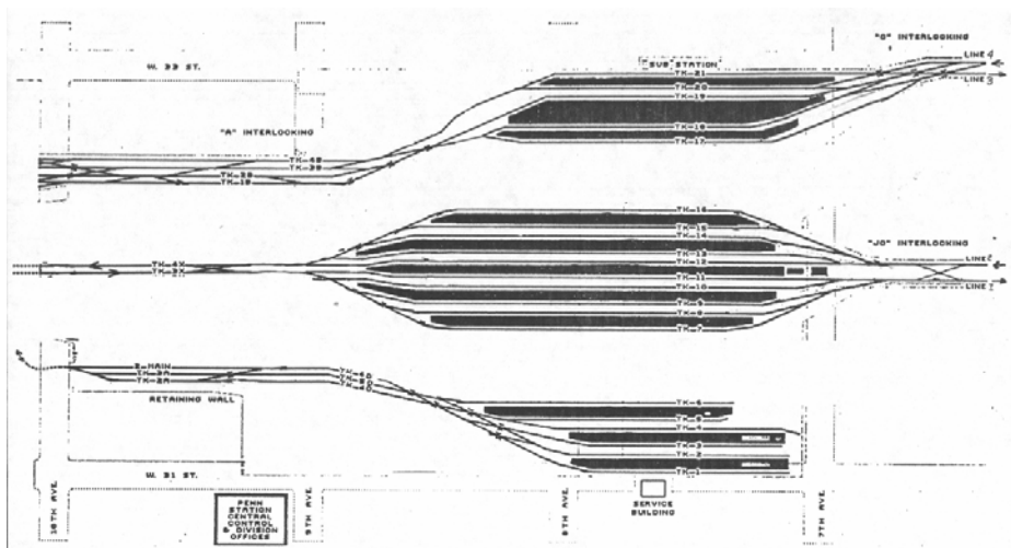
FIGURE 2 - Proposed Penn Station Metro-Hub Track Layout
