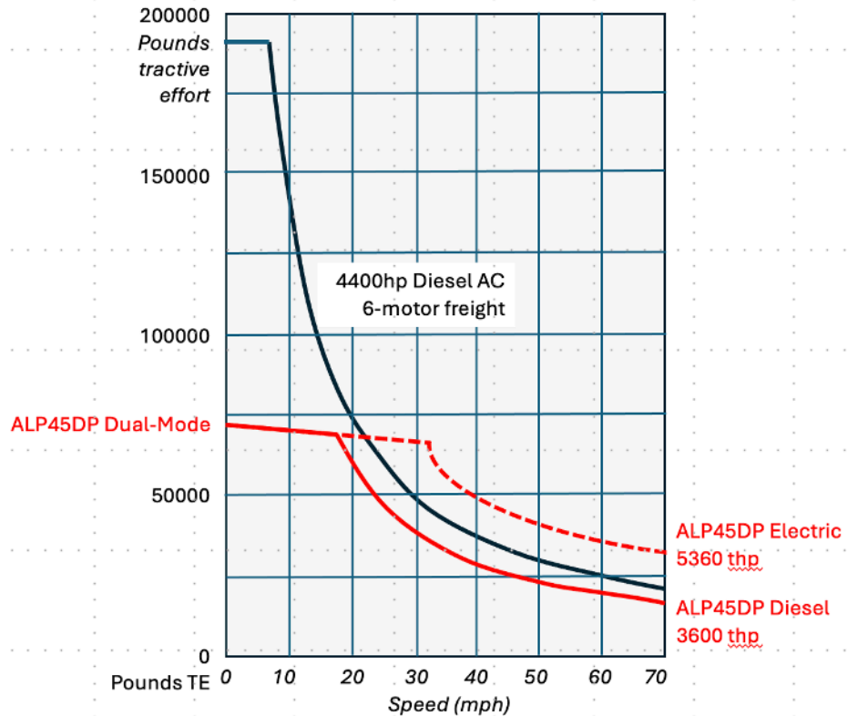
Figure 30. Tractive Effort Curve for the ALP45DP and Typical Line-haul Freight Locomotive
