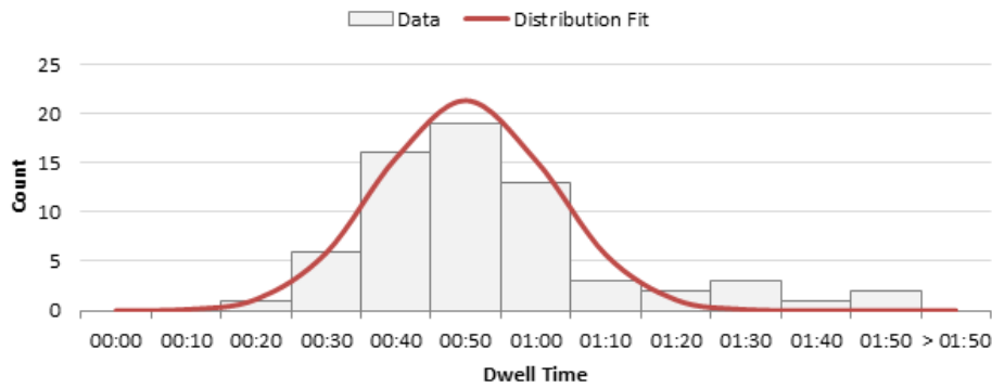
Figure 21 – Example of Normal Distribution
