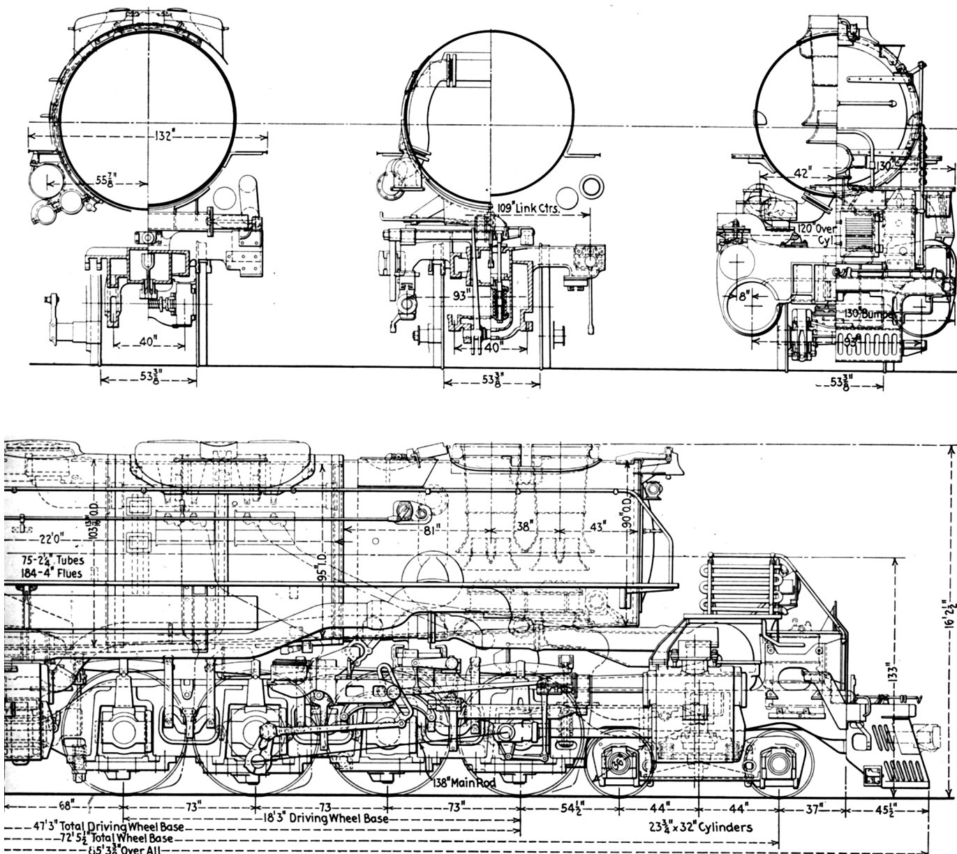
Single-Expansion Articulated Locomotives for Fast Freight Service
